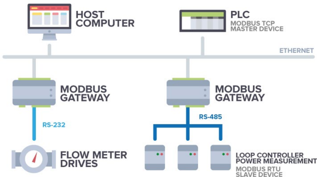
Fig. 69 Ethernet masters with multiple serial slaves
