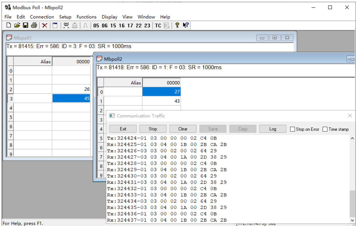
Fig. 160 Modbus RTU response
