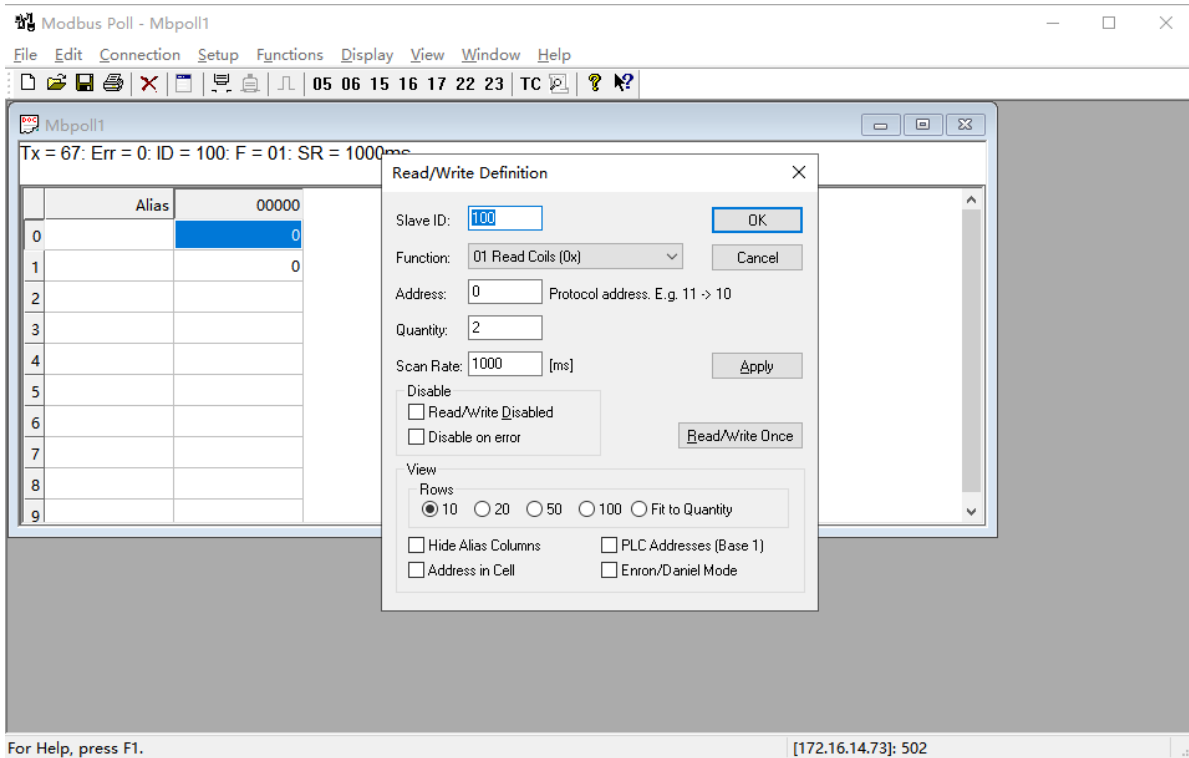
Fig. 171 Slave ID and register address
