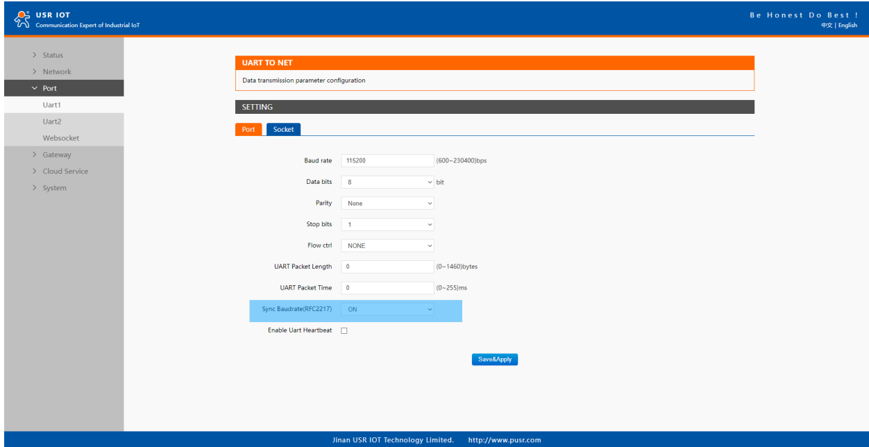
Fig. 66 RFC2217 enabled
