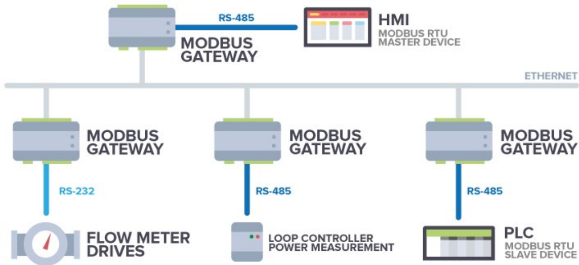
Fig. 75 Serial master with multiple serial slaves
