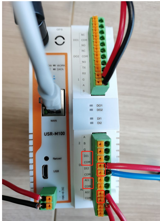
Fig. 10 Hardware connection
