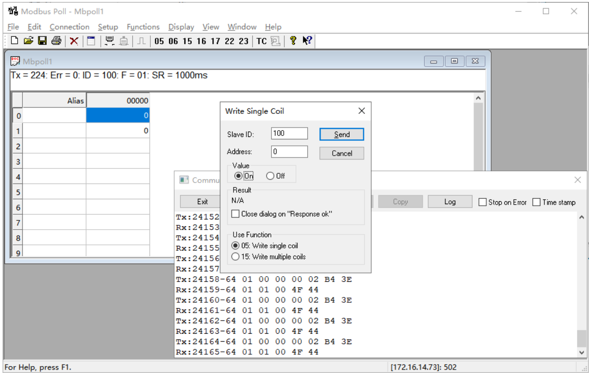
Fig. 179 Write DO
